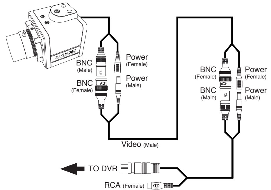
FIG. 10 Front Camera Installation
