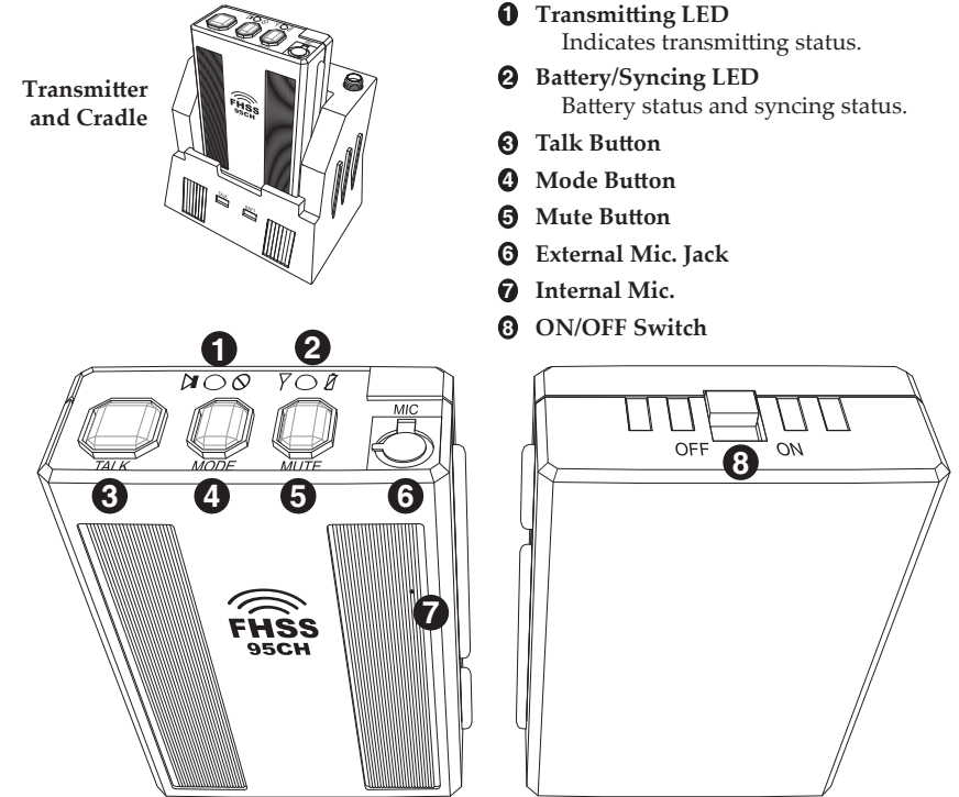
FIG. 14 2.4 GHZ Wireless Mic System
