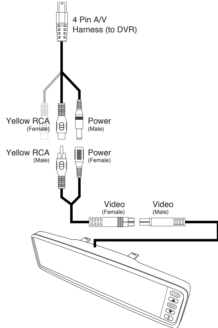
FIG. 8 Mirror Installation
