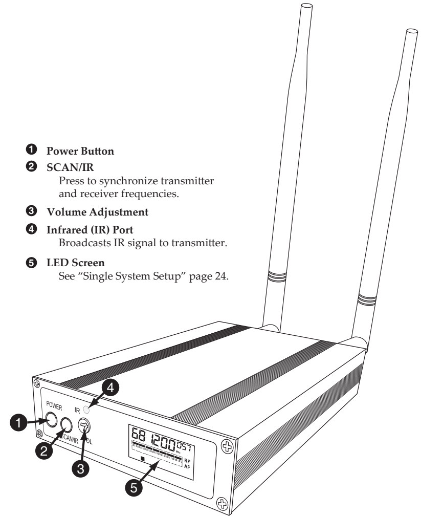
FIG. 4 UHF Wireless Receiver - FRONT
